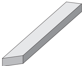
1 x C1 | 654 x 38 x 28mm | ID 20689
