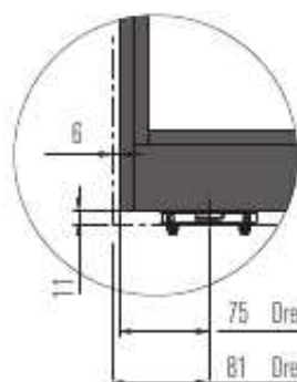
Slim Plus-Pivotband System One
